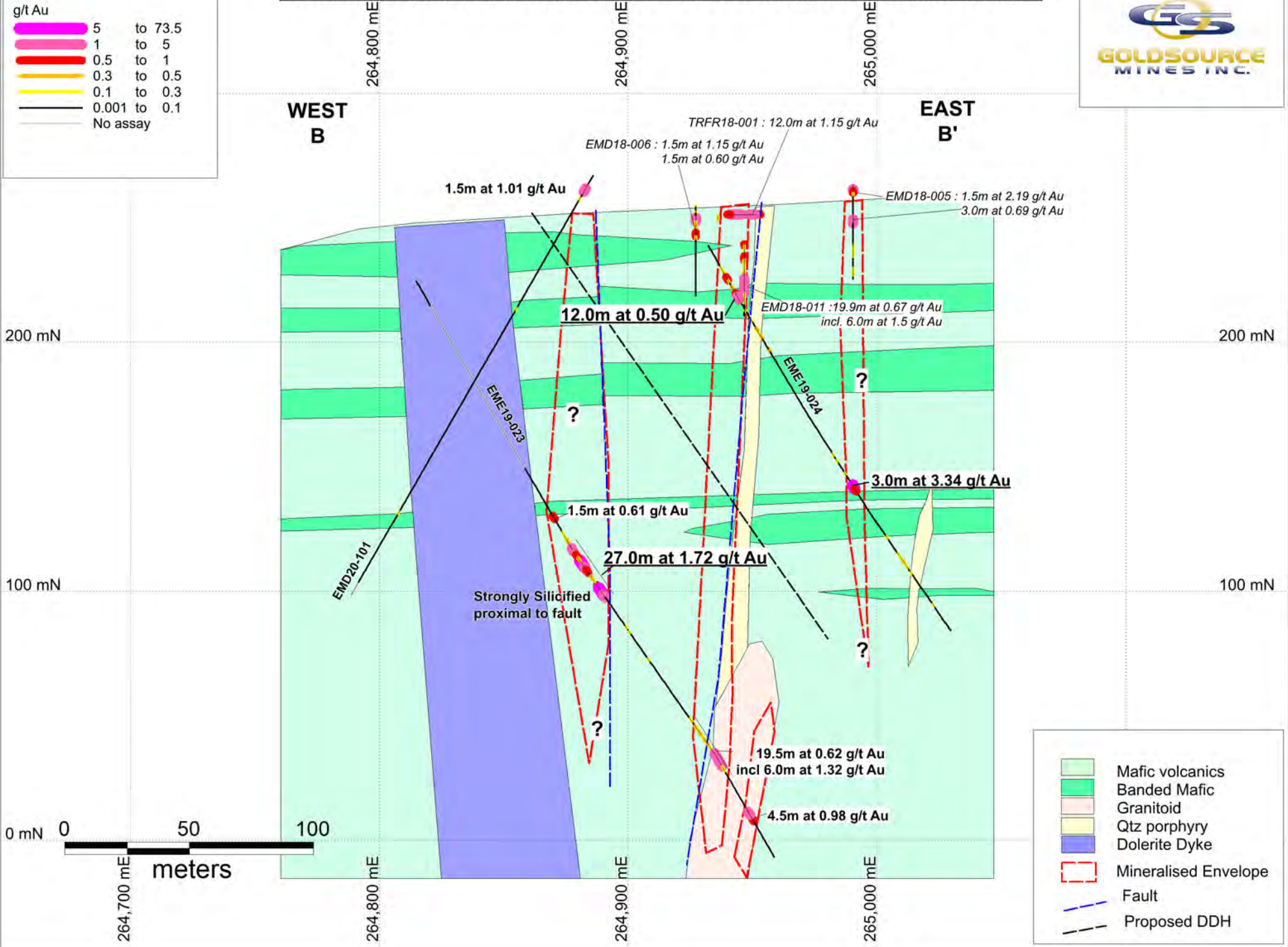
FIGURE 5 : FRIENDLY NORTH SLOPES CROSS SECTION - LOOKING NORTH
