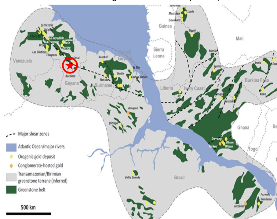
Pangean Reconstruction (120Ma) (1)
